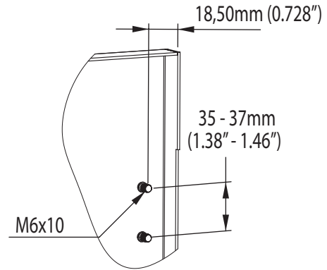
Bolt pattern for the door
